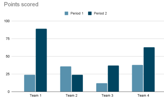
Figure 1: Points Scored
